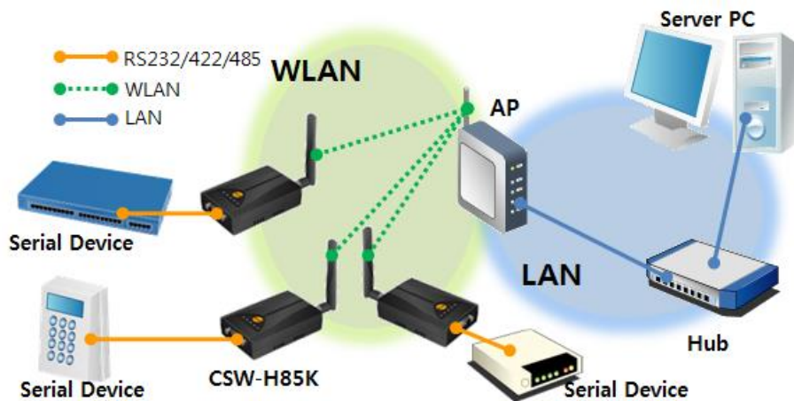
图 2-1 Infrastructure Mode
