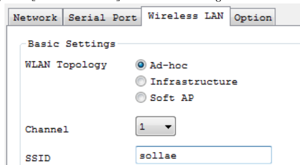
图 2-3 setting of Ad-hoc
