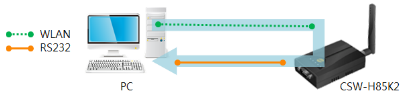
图 2-17 WLAN → RS232
